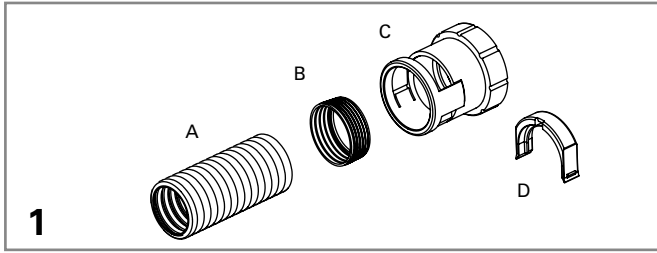
A. Conduit B. Ex Seal cap (yellow) C. Fitting D. Oval clip
