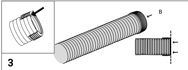
Push seal cap (B) completely onto conduit in order to achieve IP68.
