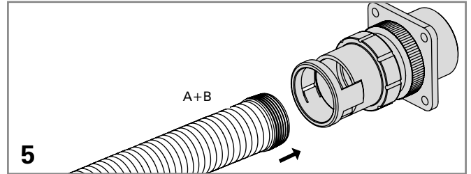
Push conduit with sealing cap (A+B) into the fitting until sealing cap is no more visible in the locking element window.
