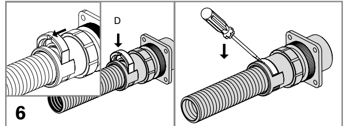
Insert Oval clip (D) in the locking element window and click into place. The screwdriver slot in the oval clip should be on the conduit side. To re-open use a screwdriver.
