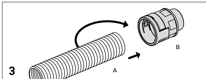
Push in the conduit (A) with a slight twist until the stop.
