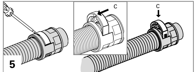
To re-open use a screwdriver. The screwdriver slot at the oval clip (C) must point towards the conduit.
