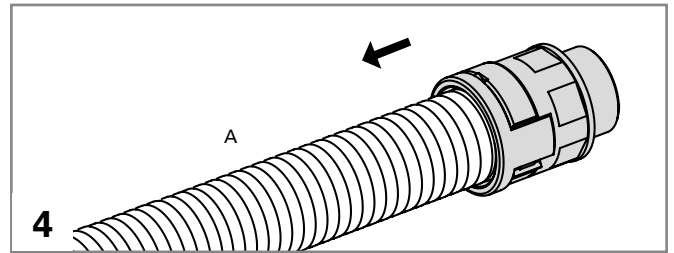
Pull back the conduit (A) slightly to ensure the locking mechanism is fully engaged.
